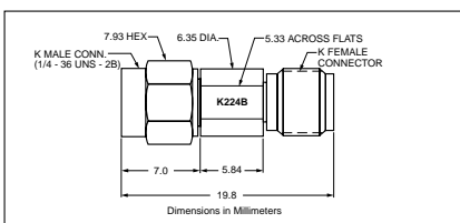
K224B Outline
