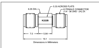
K222B Outline
