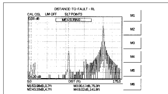
Distance-to-fault
