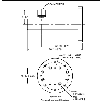
35UM48N outline
