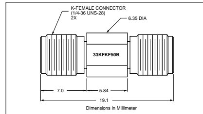
33KFKF50B Outline
