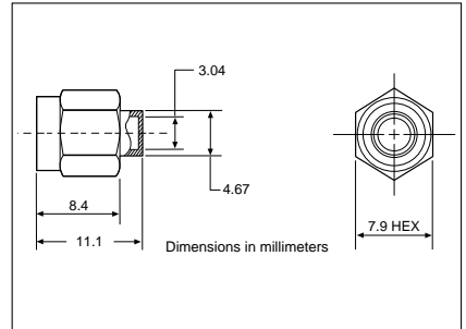
● K102F K female sparkplug launcher connector, DC to 40 GHz
