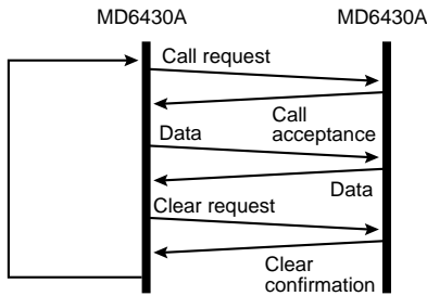
Frame relay measurement sequence
