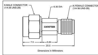
33KKF50B Outline
