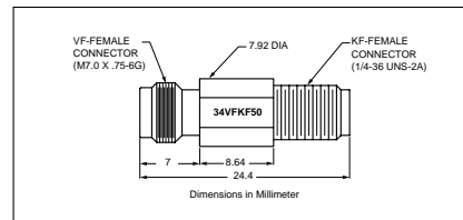
34VFKF50 Outline
