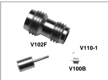
• V202FB Combination of V102F, V100B, V110-1
