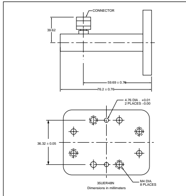
35UER48N outline
