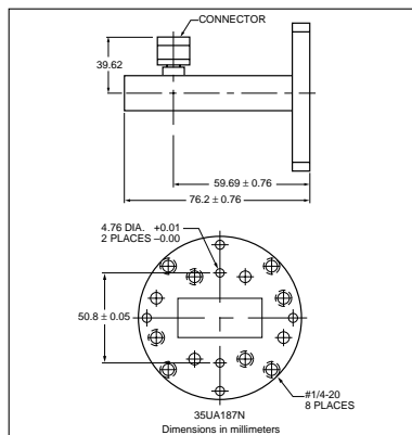
35UA187N outline
