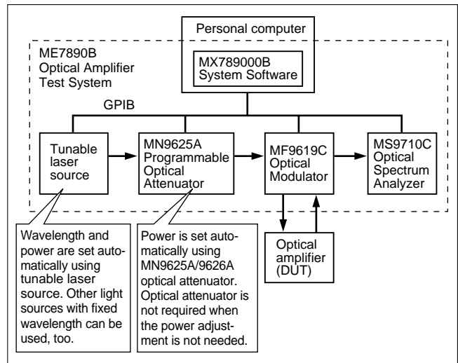
System setup
