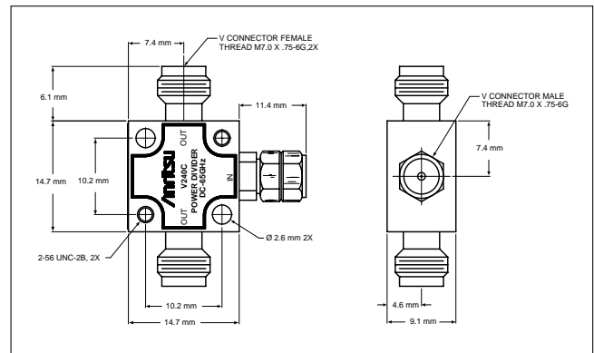
V240C outline
