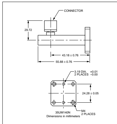
35UM140N outline
