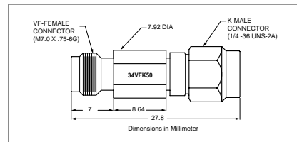
34VFK50 Outline
