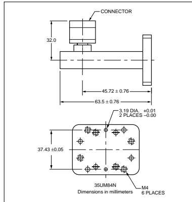
35UM84N outline
