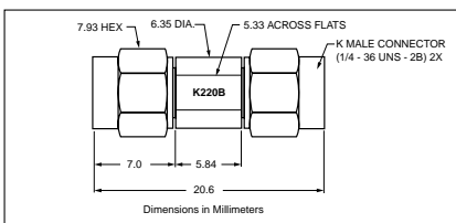
K220B Outline
