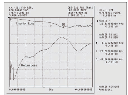
Insertion Loss and Return Loss measured on K261 over the range of 40 MHz to 40 GHz. K261 DC Block Return Loss
